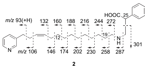
Figure 5. Fragmentation patterns of nakinadine C ( 2 ) in ESIMS/MS [parent ion; at m/z 437 ( M+H ) ^+ ].
