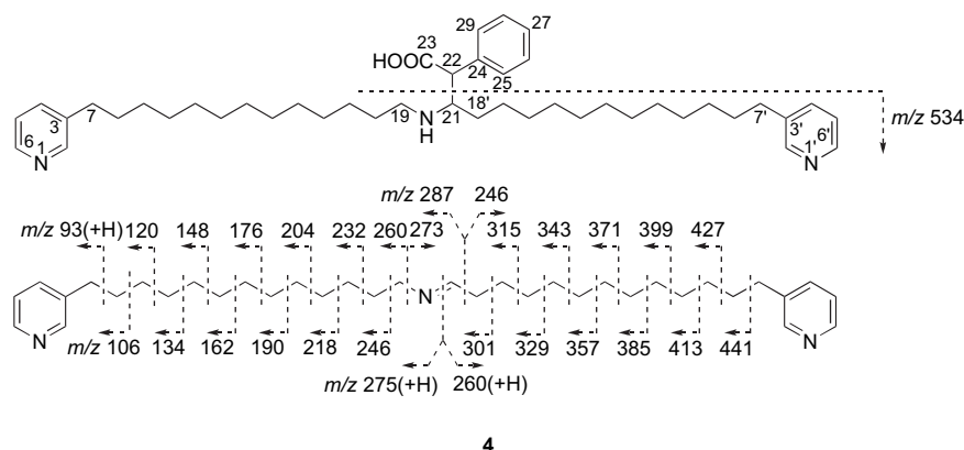
Figure 8. Fragmentation patterns of nakinadine E ( 4 ) in ESIMS/MS [parent ion; (A) at m/z 670 ( M+H ) + , (B) at m/z 534 ( M-C_8H_9O_2+H ) + ].
