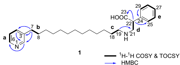
Figure 1. Selected 2D NMR correlations for nakinadine B ( 1 ).
