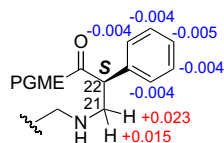
Figure 3. \Delta\delta values [ \Delta\delta (in ppm) \delta_S - \delta_R ] obtained for ( S )- and ( R )-PGME amides of nakinadine B ( 1 ).
