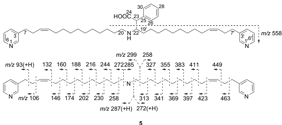
Figure 9. Fragmentation patterns of nakinadine F ( 5 ) in ESIMS/MS [parent ion; (A) at m/z 694 ( M+H ) + , (B) at m/z 558 ( M-C_8H_9O_2+H ) + ].
