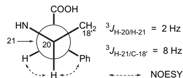
Figure 7. Rotation model for C-20 to C-21 of nakinadine D ( 3 ).
