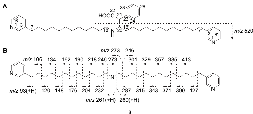
Figure 6. Fragmentation patterns of nakinadine D ( 3 ) in ESIMS/MS [parent ion; (A) at m/z 656 ( M+H ) ^+ , (B) at m/z 520 ( M-C_8H_9O_2+H ) ^+ ].
