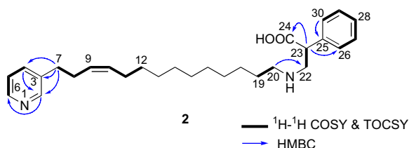
Figure 4. Selected 2D NMR correlations for nakinadine C ( 2 ).
