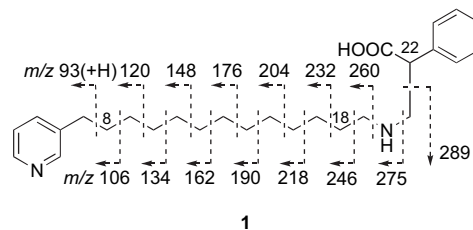
Figure 2. Fragmentation patterns of nakinadine B ( 1 ) in ESIMS/MS [parent ion; at m/z 425 ( \text{M}+\text{H}^+ )].
